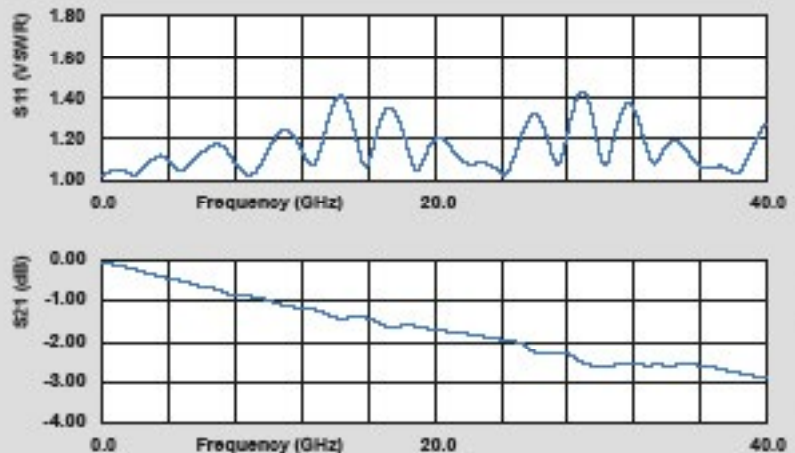
1" microstrip test board with typical data through 40 GHz
